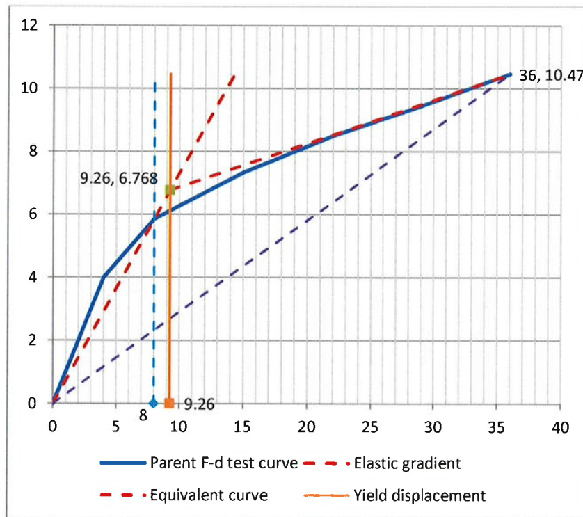
Figure 1: Equivalent Bi-linear elasto-plastic curve, 1200mm long Metalcraft test panel
